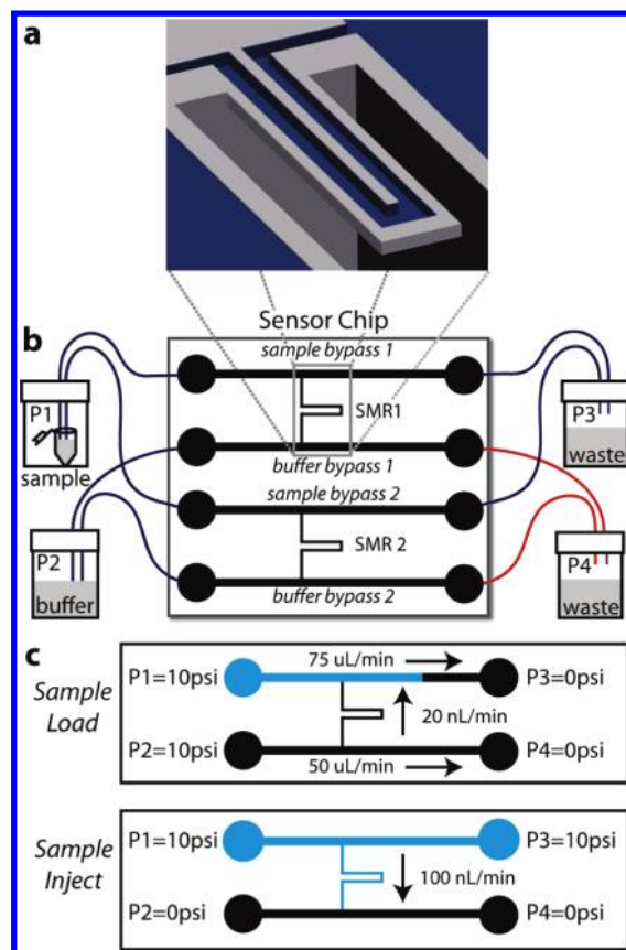
Figure 1. Suspended microchannel resonator (SMR) system schematic. (a) Cut-away view of SMR microcantilever. The U-shaped sensor channel has a 3 \times 8 \mu\text{m}^2 cross section and is embedded in a resonating silicon beam extending 200 \mu\text{m} into a vacuum-packaged cavity. (b) Sensor chip with two SMRs addressable by bypass channels connected by Teflon tubing to pressure-controlled vials off-chip; one SMR is used as a control (reference) sensor: blue tubing, i.d. 225 \mu\text{m} ; red tubing, i.d. 150 \mu\text{m} . (c) Fluid delivery schemes: “Sample Load” fills sample bypass channels with sample (blue) while the microcantilevers and buffer bypasses are flushed with running buffer (black); “Sample Inject” delivers a sharp concentration sample to the microcantilevers. Figures are not to scale.
